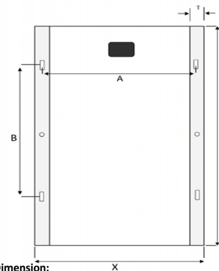
Mechanical Dimension:
